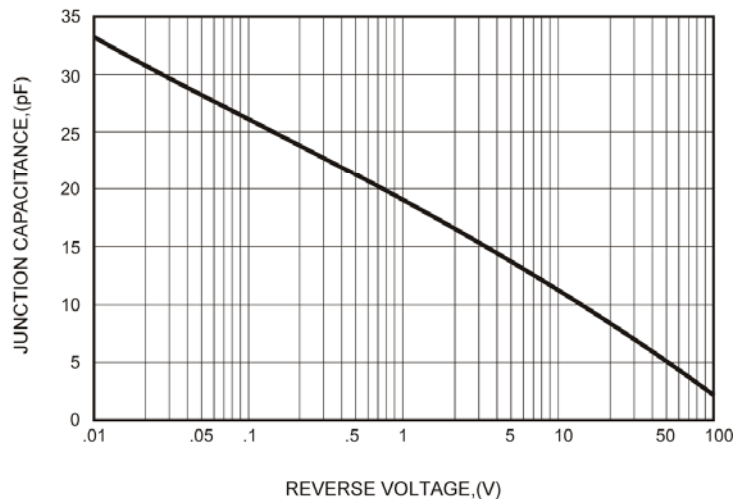
FIG.5-TYPICAL JUNCTION CAPACITANCE
